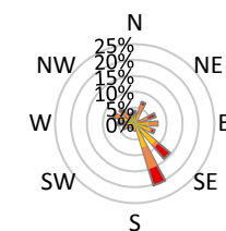
PM 2.5 Pollutant Rose
