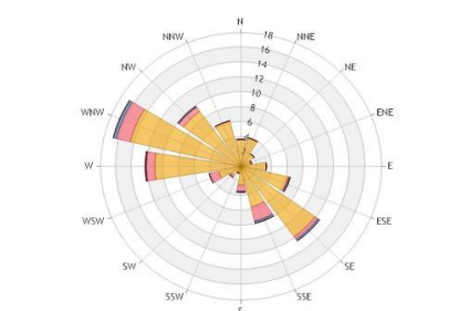
SO 2 Pollution Rose
