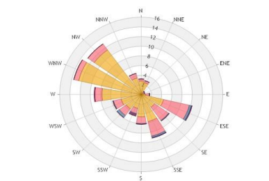
NO 2 Pollution Rose
