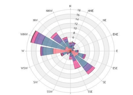
O 3 Pollution Rose
