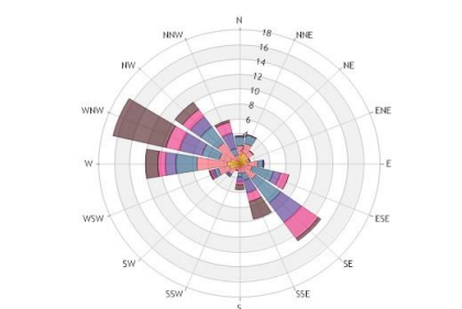
Wind Rose
