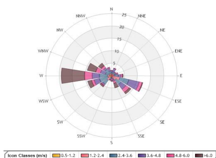
Wind Rose
