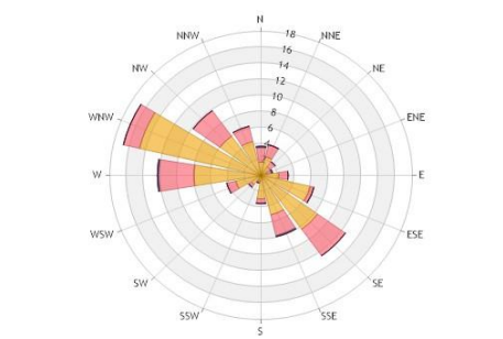
H 2 S Pollution Rose
